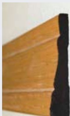
COLONIAL DOOR & WINDOW CASING STANDARD Oak \frac{1}{2}" \times 2\frac{1}{4}" Painted \frac{9}{16}" \times 2\frac{1}{4}" Pine \frac{11}{16}" \times 2\frac{1}{4}" Hickory \frac{1}{2}" \times 2\frac{1}{4}"
